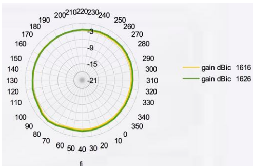
GAIN AZIMUTHAL
