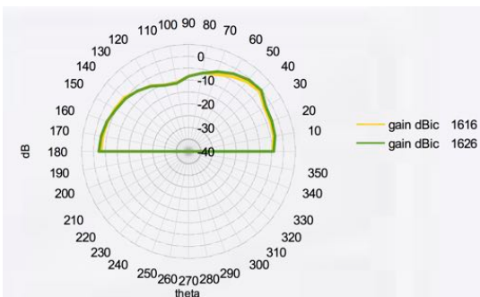
GAIN AZIMUTHAL
